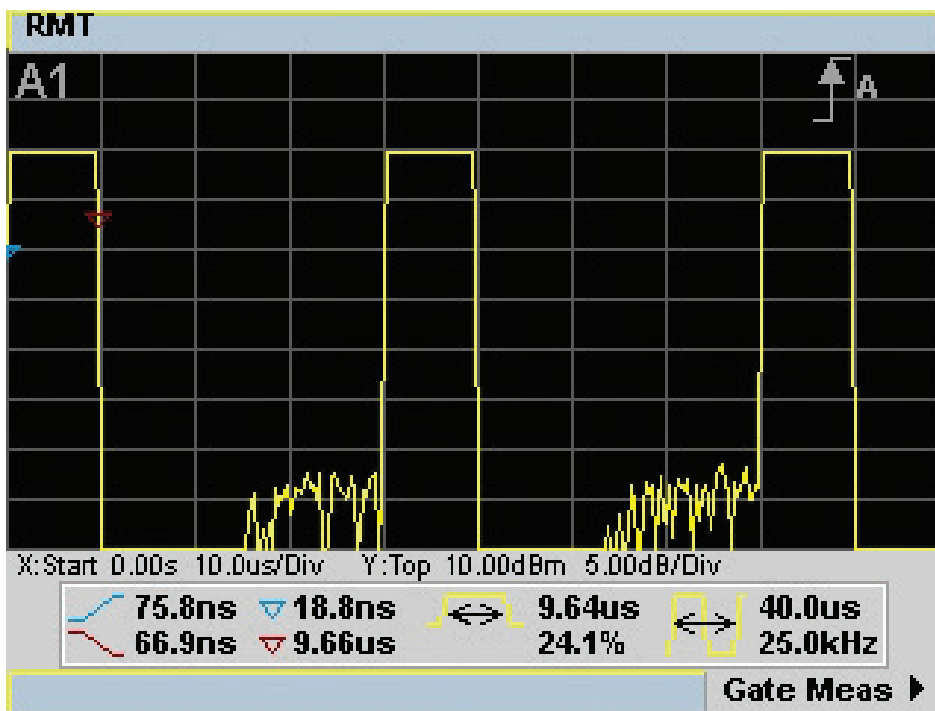
Figure 10. The P-Series peak power meter will automatically measure pulse characteristics including rise time, fall time, pulse width, and pulse period.
