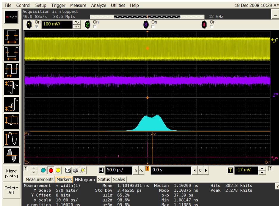
Figure 37. The built-in capabilities of the DSO90000 series make it possible to acquire a chirped radar pulse with a bimodal PRI and then display a histogram of thousands of pulses.
