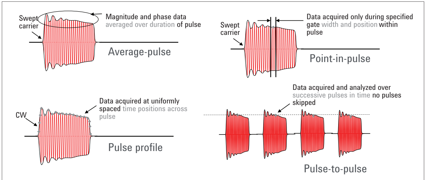
Figure 43. For radar applications, the Keysight PNA has four different pulse-sampling options
