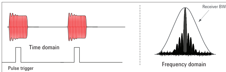
Figure 39. Wideband detection mode (synchronous detection mode) of a network analyzer requires the majority of the pulse power be contained within the receive bandwidth of the network analyzer. Wideband mode may have the best dynamic range for signals with low duty cycle but will be limited in measurable pulse widths due to bandwidth constraints.
