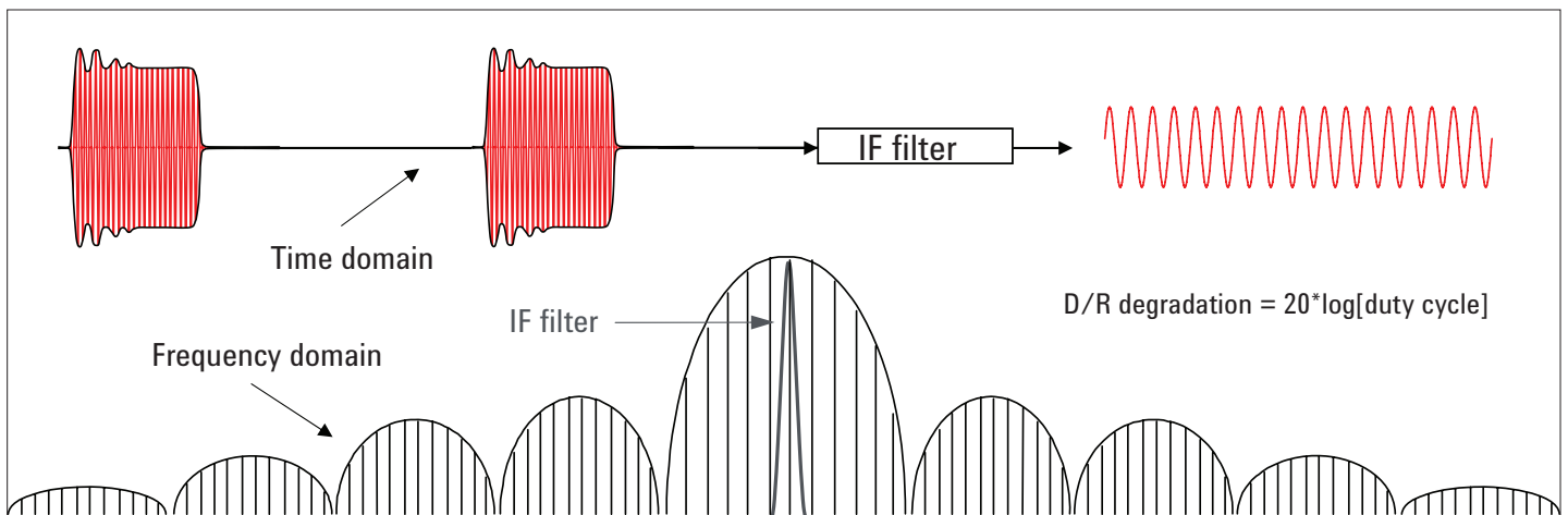
Figure 40. The narrowband detection mode (asynchronous detection mode) of a network analyzer uses a narrow filter to extract only the central spectral component. The narrowband mode has no pulse width limitations.
