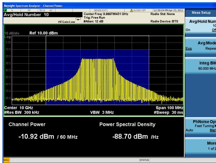
Chirped radar
