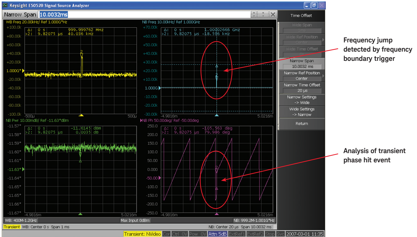
Figure 61. The SSA includes time-domain analysis and advanced trigger functions useful for examining transient events. In this screen, the analyzer is able to use its frequency-boundary trigger to capture and analyze a phase hit.
