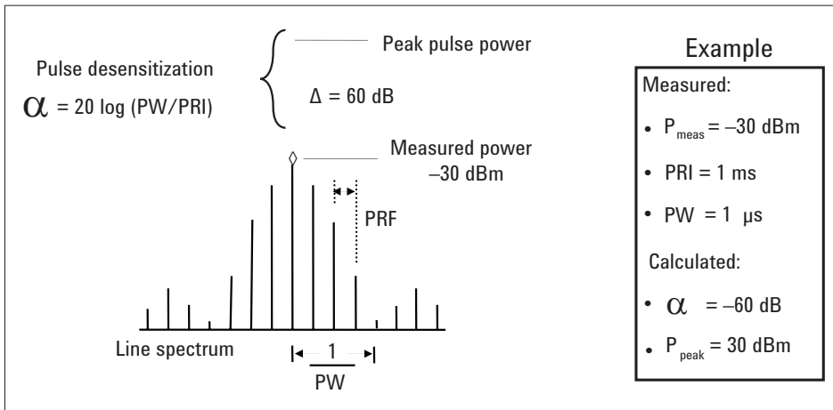
Figure 19. Calculating peak power from the pulsed RF spectrum (line mode) using the pulse desensitization factor.
