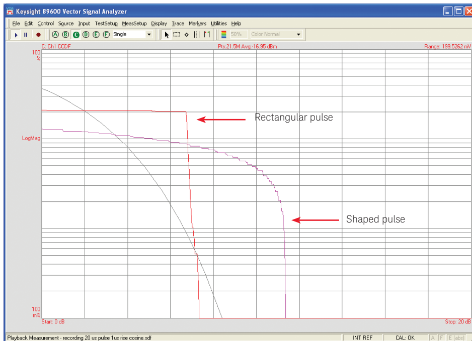
Figure 35. CCDF measurement of a square pulse radar signal compared to a raised-cosine-shaped pulse radar signal. A CCDF plot describes the power statistics of a signal by plotting the percentage of time (y axis) the signal spends at x dB above the average power (x axis).
