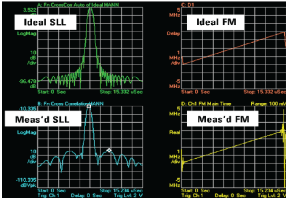
Figure 55. Example SLL measurements made with the 89600 VSA software
