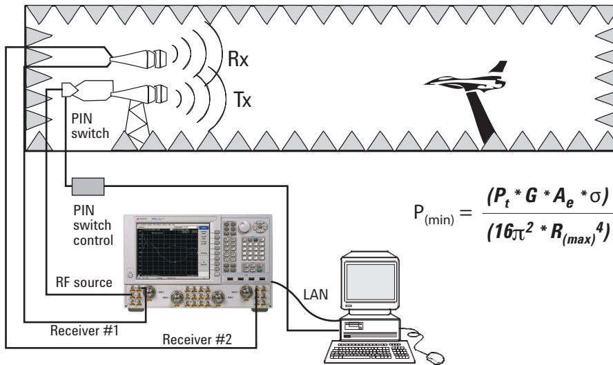
Figure 52. This example radar cross section measurement setup uses a network analyzer and an anechoic chamber.
