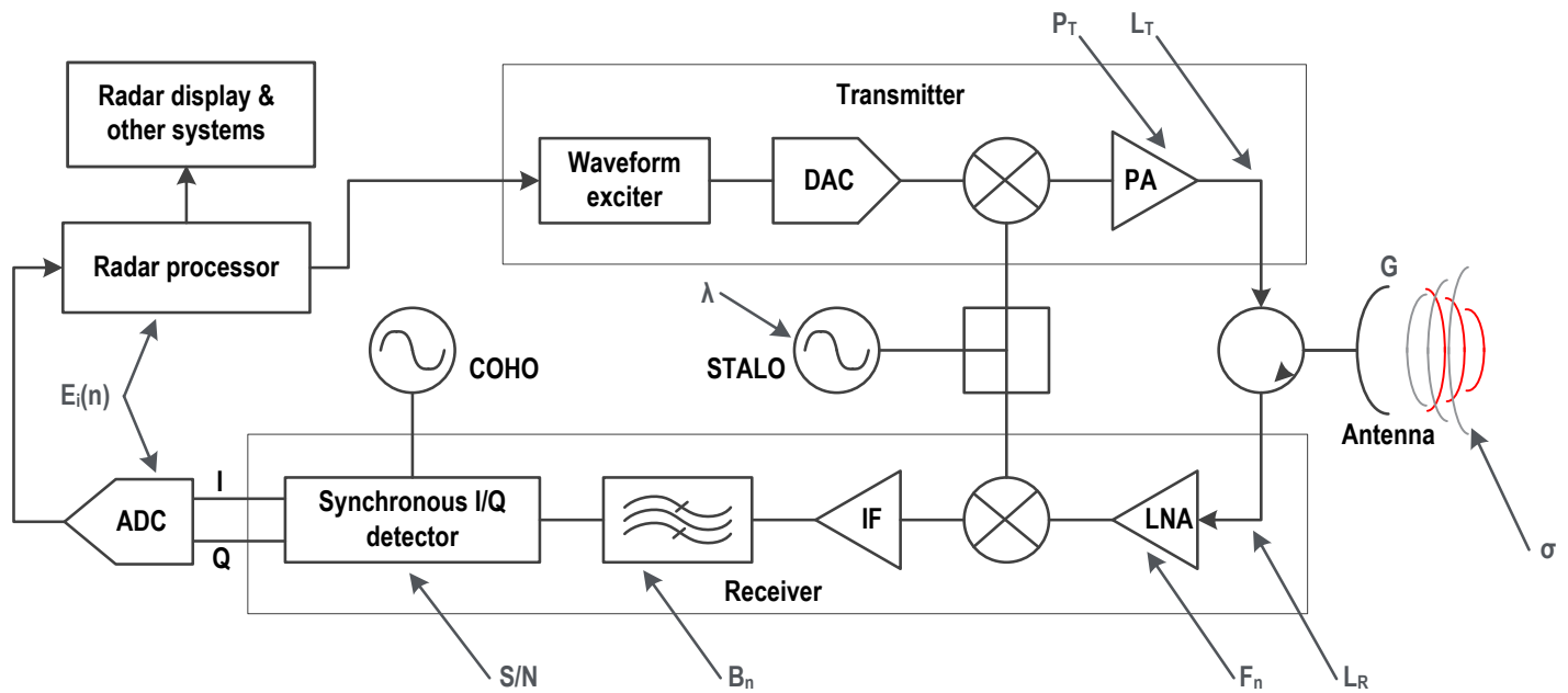
Figure 5. Relating key variables in the radar range equation to hybrid analog/digital implementations of the transmitter and receiver sections of a radar system
