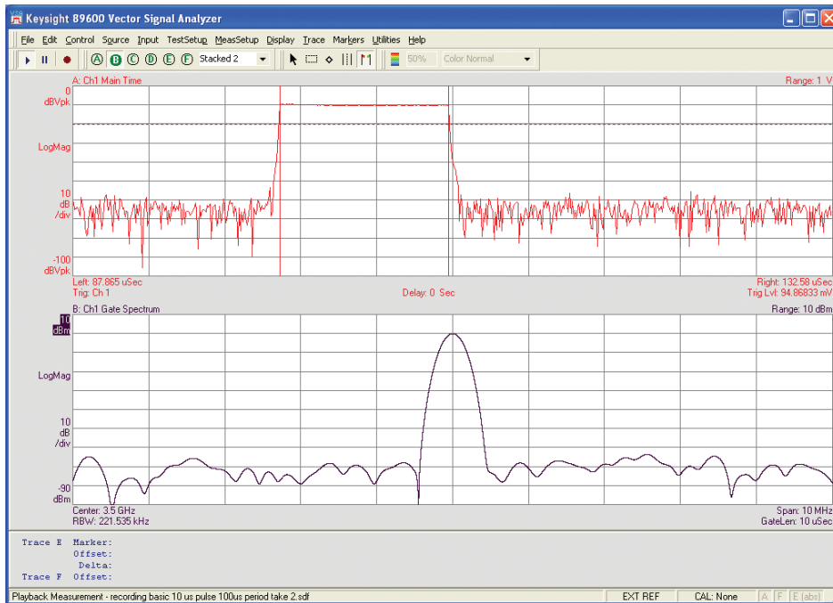
Figure 32. This is a time-gated measurement of simple RF pulse showing CW spectrum of signal when pulse is on.
