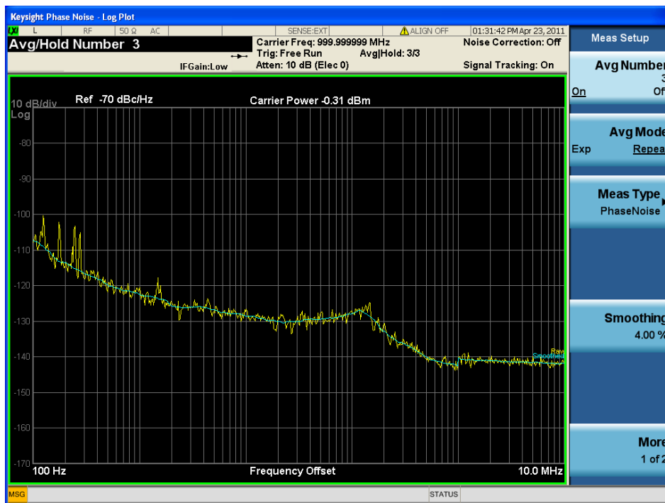
Figure 58. With the PXA spectrum analyzer phase noise measurement application, results are displayed as a function of offset frequency from the carrier
