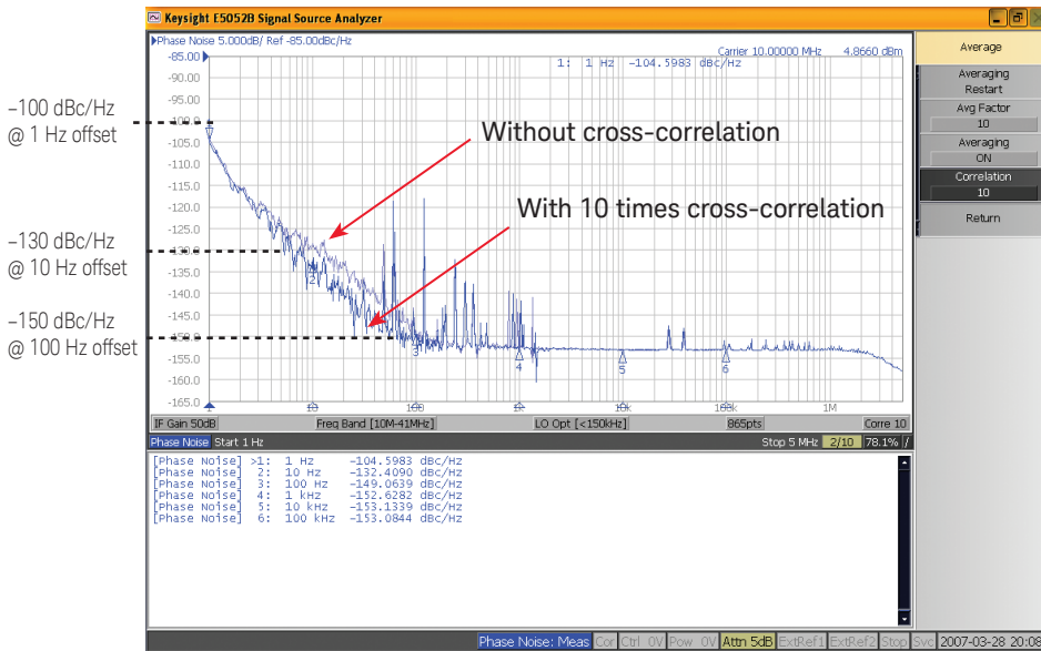
Figure 60. This phase noise measurement uses Keysight's signal source analyzer (SSA). The phase noise measurement is improved using a cross-correlation technique.
