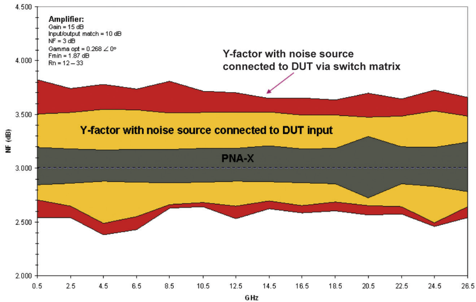
Figure 54. PNA-X-based noise figure solution provides the best measurement uncertainty due to its high sensitivity and ability to use vector error corrections to subtract errors due to effects such as impedance mismatch.
