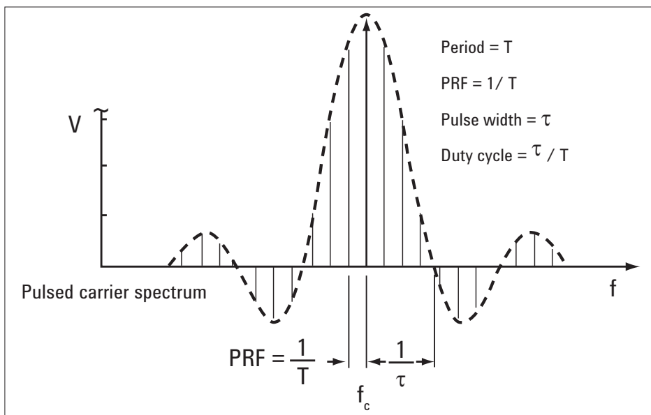
Figure 17. Pulsed spectrum
