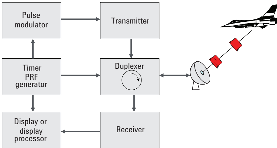
Figure 4. Basic radar block diagram
