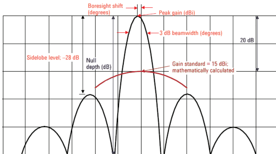
Figure 44. Many importance characteristics of the antenna can be determined from the antenna pattern.
