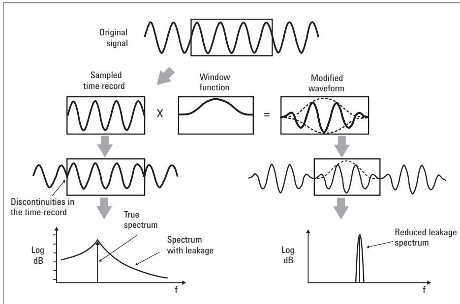
Figure 29. FFT analysis done in a spectrum analyzer or vector signal analyzer assumes a repeating signal. To minimize effects of discontinuities in the signal, a windowing function is used.
