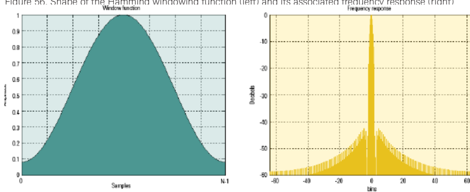
Figure 56. Shape of the Hamming windowing function (left) and its associated frequency response (right)
