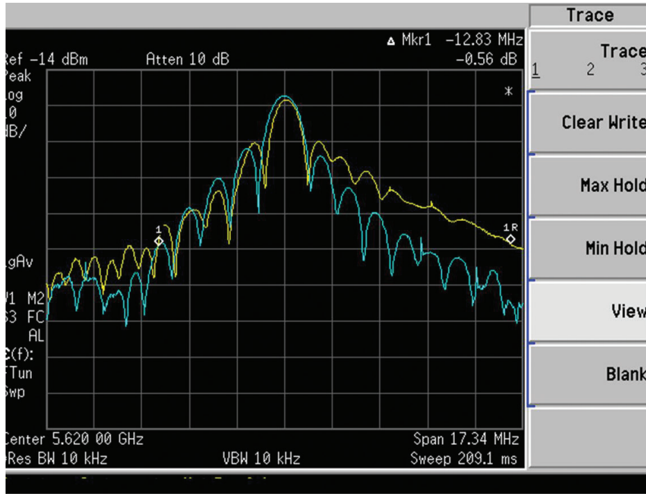
Figure 16. A signal analyzer is useful for examining the shape and symmetry of the radar spectrum. This example shows the spectrum trace before and after a timing adjustment in the magnetron.
