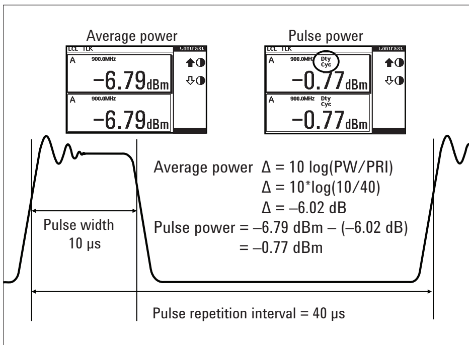
Figure 7. Using an average power meter to derive pulse power.
