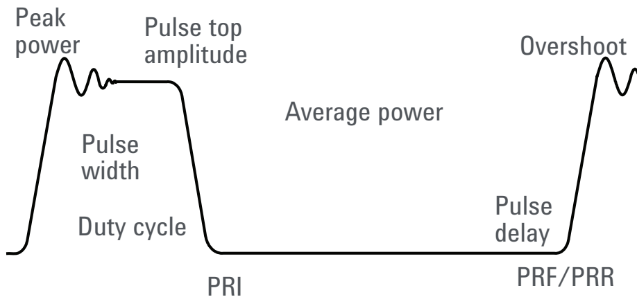
Figure 6. Pulse parameters
