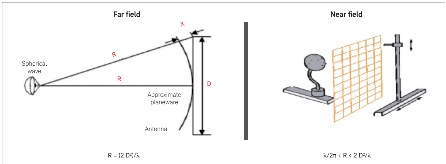
Figure 45. Antenna measurements can be made using either a far-field or near-field approach. Far-field testing is simpler and faster but requires a large area. Near-field testing requires sophisticated calculations and may take longer to perform, but requires less space.
