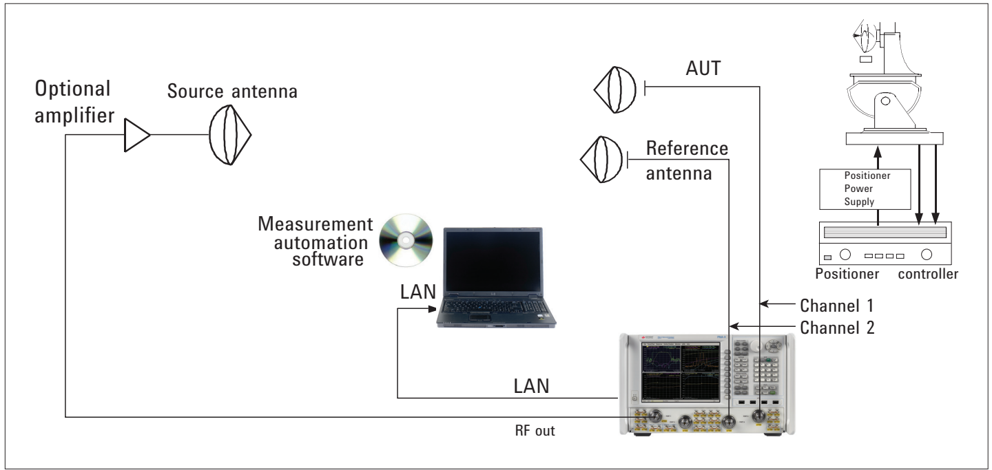
Figure 47. This example of a simple test configuration with a network analyzer is used for smaller far-field test setups, but may not be possible for large ranges due to cable losses.
