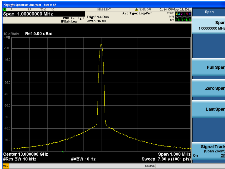
Figure 57. Phase noise results in sidebands that spread power into adjacent frequencies reducing the signal-to-noise ratio
