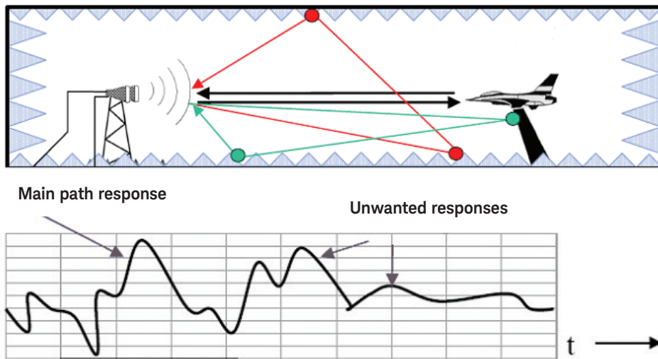
Figure 53. RCS signals are small and returns caused by the measurement chamber can interfere with the measurement results.
