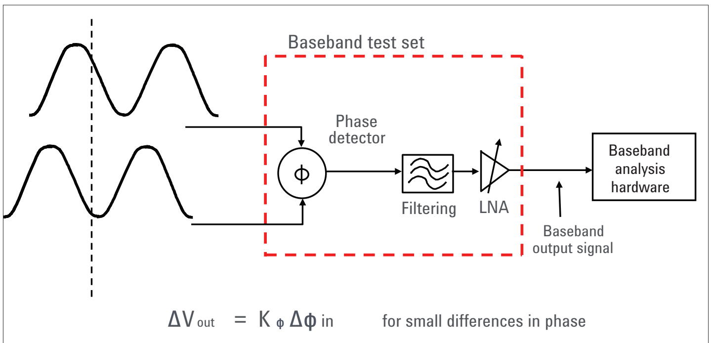
Figure 59. A basic block diagram of phase detector-based phase noise measurement. The measurement compares the test signal to a phase-locked reference signal with a phase detector. Variations in phase due to phase noise result in a voltage output that is then processed to determine the phase noise result.
