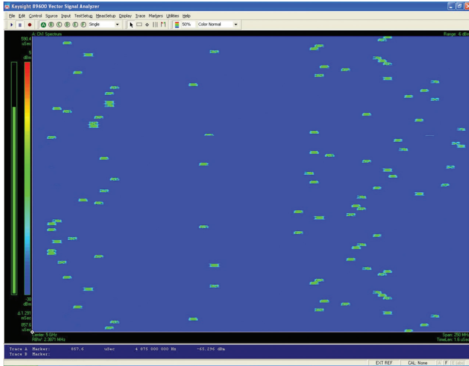
Figure 33. Spectrogram showing frequency agile signal over 1 GHz span, made with 89600 VSA software running on a 90000 series oscilloscope.
