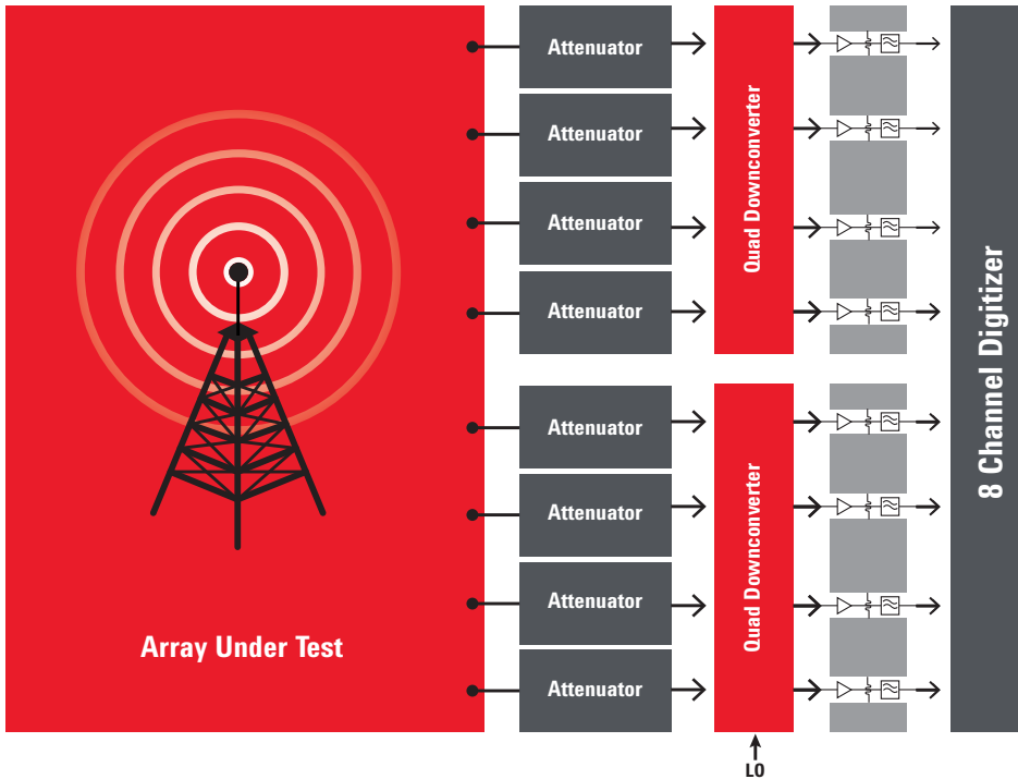
Figure 51. This generic configuration enables rapid phase-coherent test and calibration of multi-antenna arrays.
